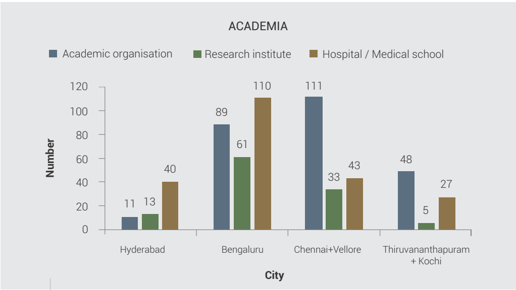
Figure 2.2 | Distribution of academic institutes in four south Indian clusters
